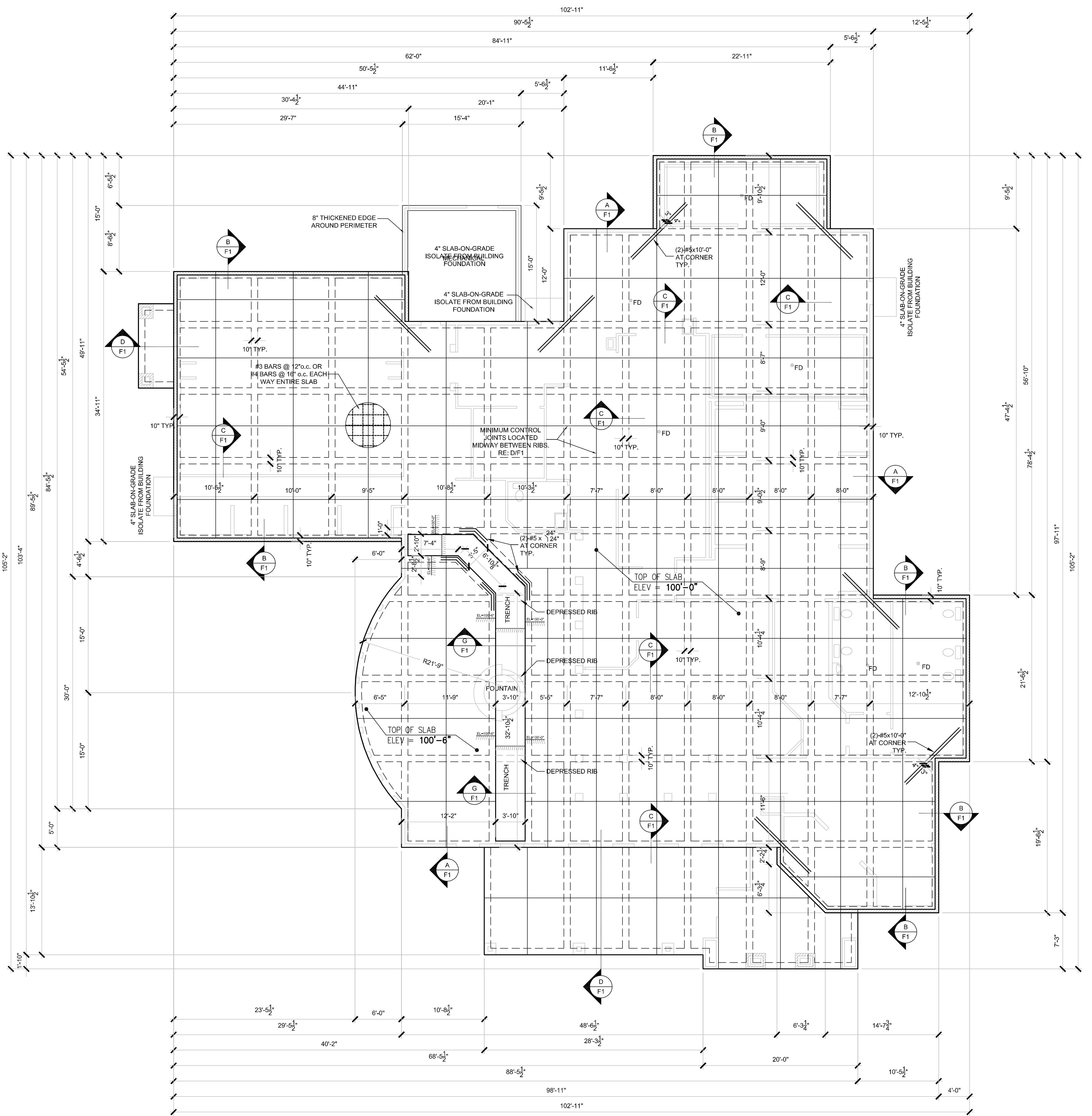
1 FOUNDATION PLAN SCALE: 1/8" = 1'-0"
